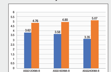
Energy Efficiency Ratio (EER) ■ 100% Capacity ■ 50% Capacity
